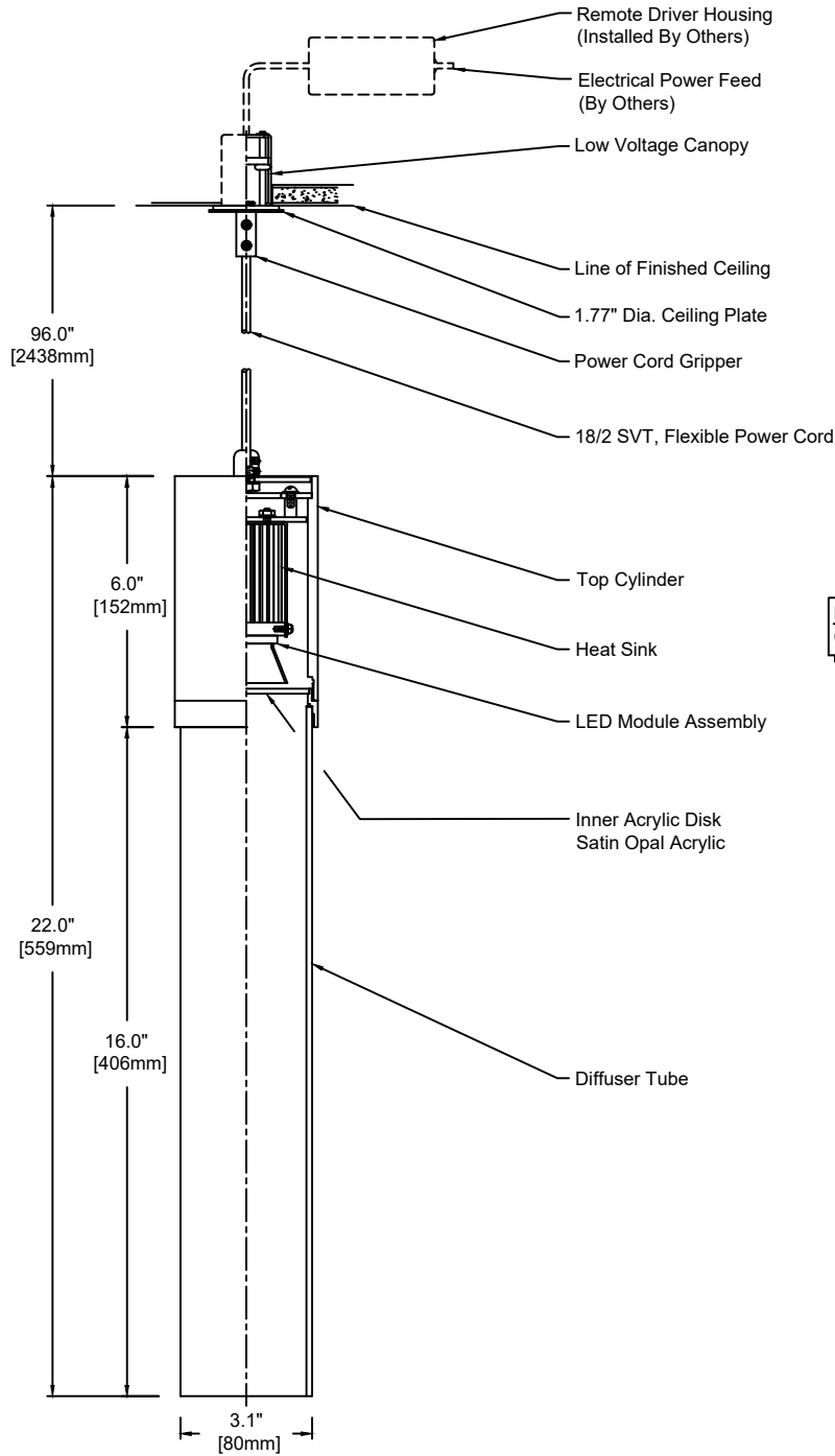
PERSPECTIVE VIEW
