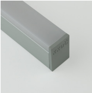
SA Silver anodised finish with grey end caps. W13/H19mm (W0.51/H0.75")
