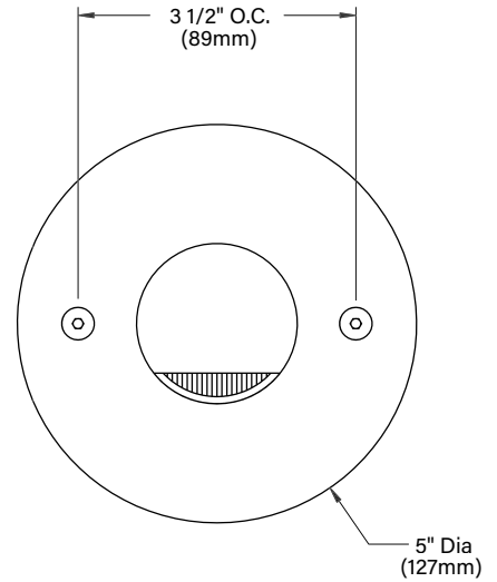
FACEPLATE DETAIL
