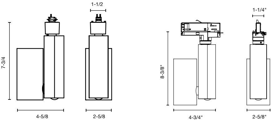
(Shown with ECO/HALO/JUNO/LGTR type adapter) (Shown with GEO type adapter)
