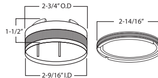
LED Holder
