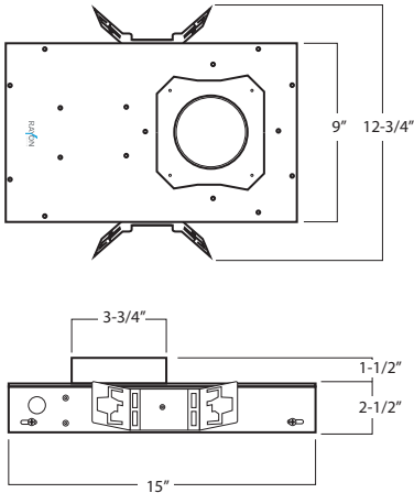
IC Housing
