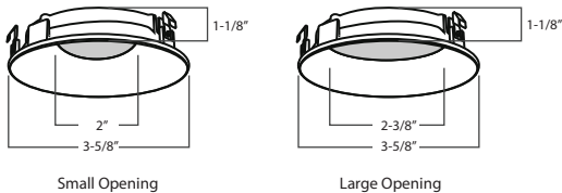
Trim
